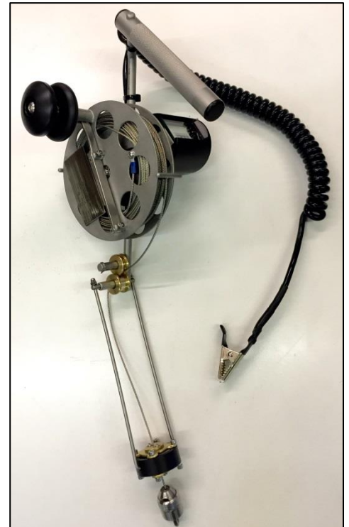
ATEX Approved MK 1A Winder with cable wiper & optional depth counter
